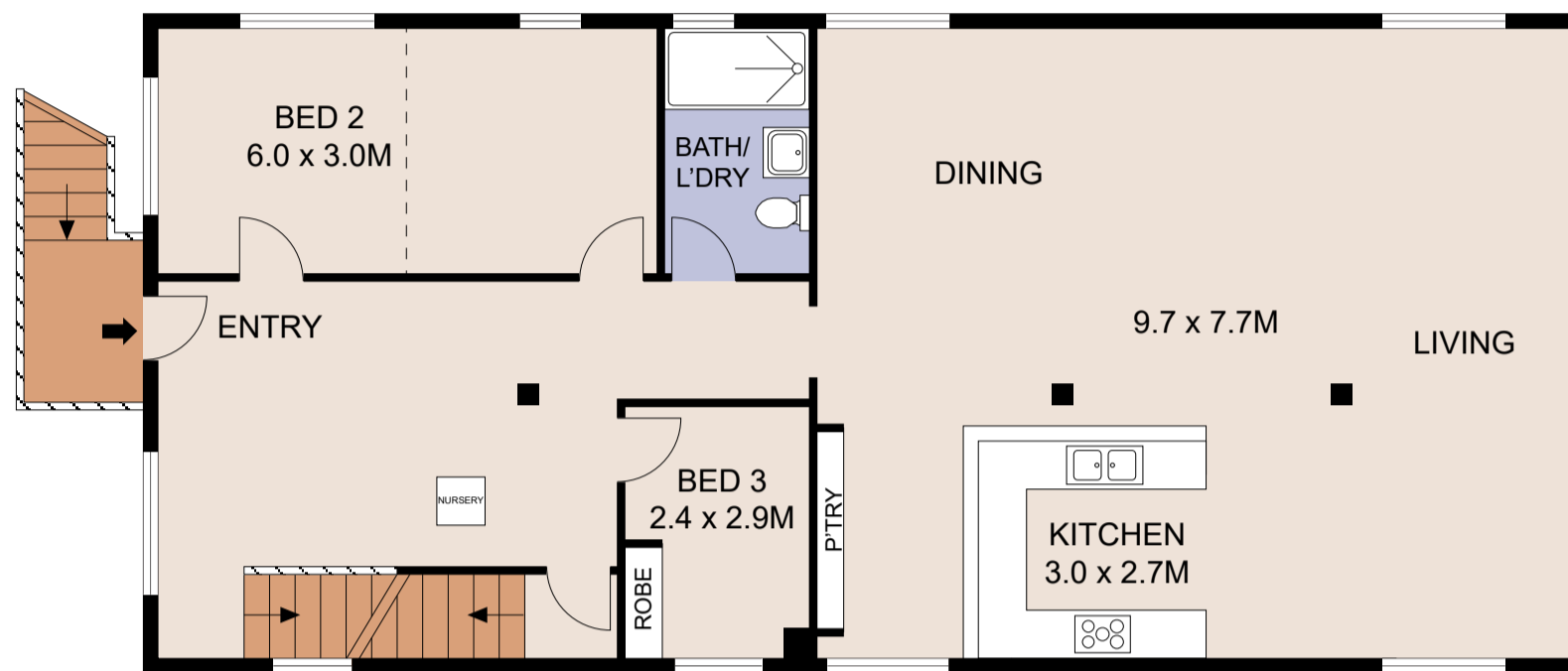
FIRST FLOOR
